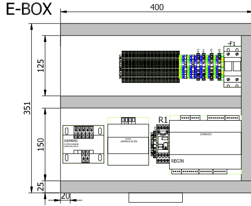
PANEL ASSEMBLY SHEET:351x400 mm CABLE DUCT:25X60 mm
